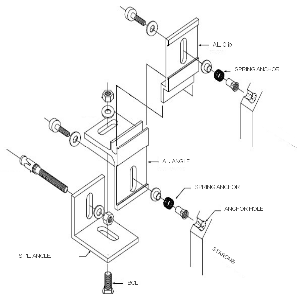
DWG 1 – Anchor Assembly
