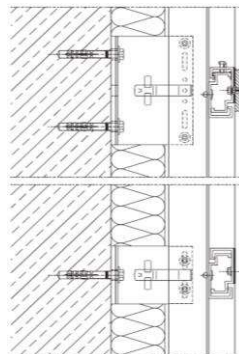
DWG 1 - Vertical
