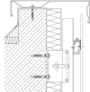
DWG 5 – Upper Ending
