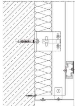
DWG 4 – Lower Ending
